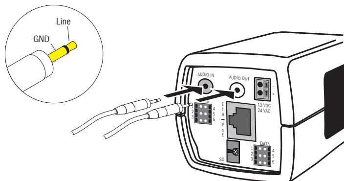
Figure 5.7 Audio connectors
